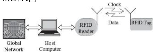
Fig. 1. Block diagram of a typical RFID system. [4]
